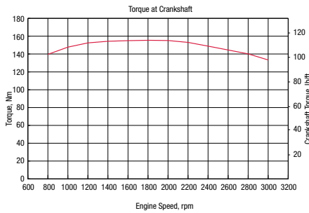
Torque
