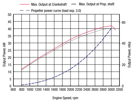
Power
