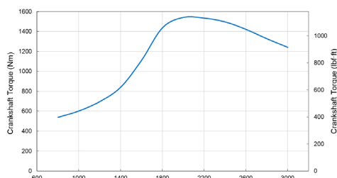
6LF550 Torque curve
