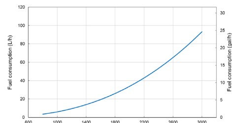
6LF530 Fuel consumption (load exp. 2.5)
