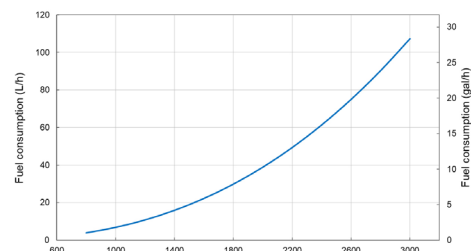
6LF550 Fuel consumption (load exp. 2.5)
