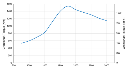
6LF530 Torque curve
