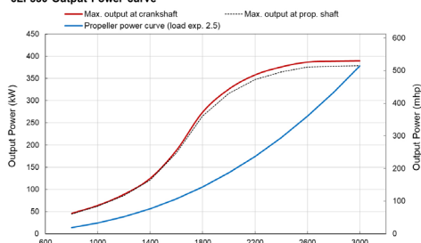
6LF550 Output Power curve
