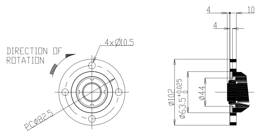
DETAIL OF COUPLING SCALE 1:3 ARROW B
