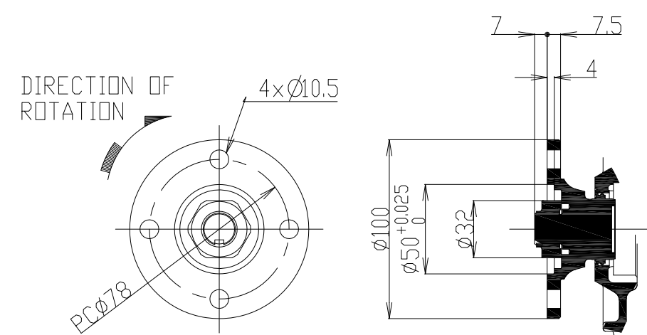
DETAIL OF COUPLING SCALE 1:3 ARROW B
